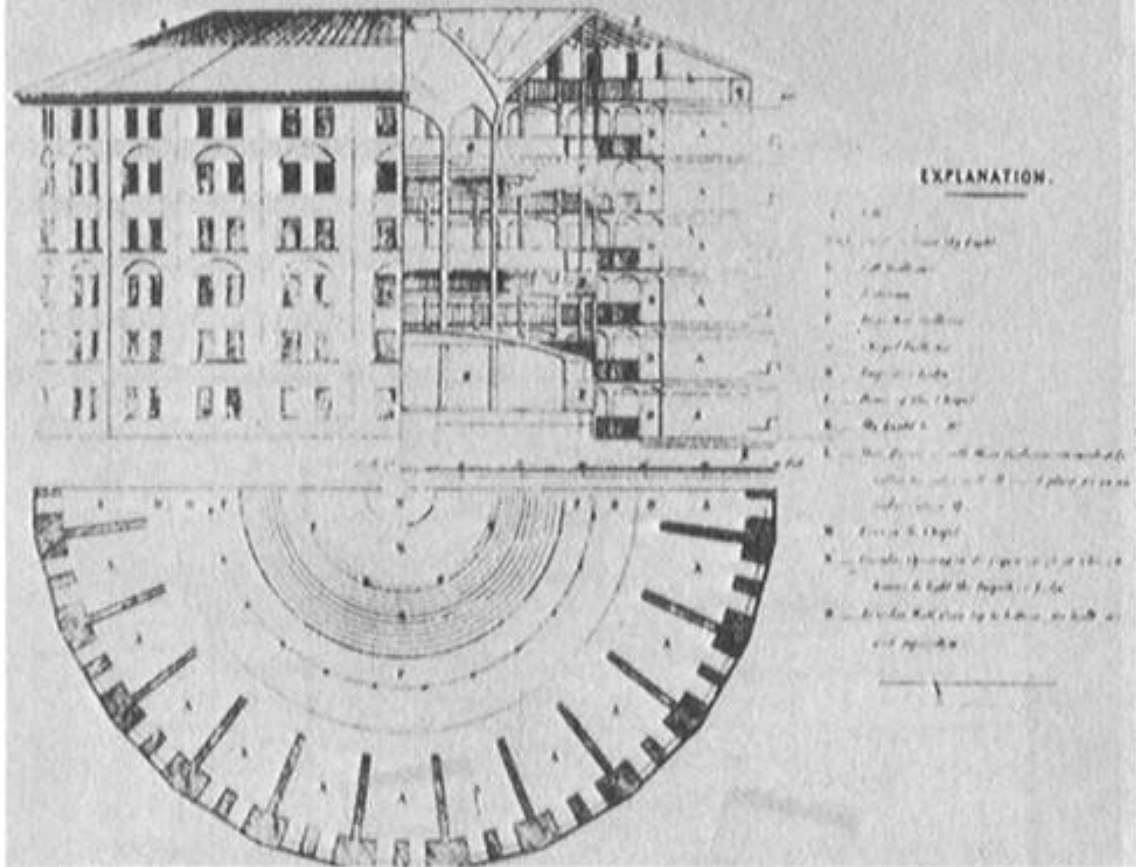
A General Idea of a PENITENTIARY PANOPTICON in an improved, but as yet unfinished, State. See Postscript Reference to Plans, Elevation & Section (being Plans referred to as N o 1).
