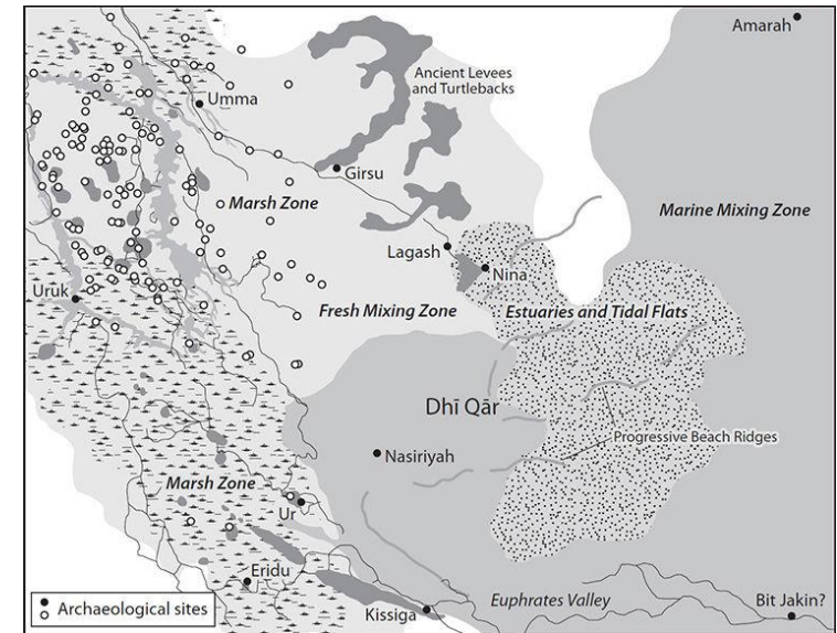
Figure 9. Southern Mesopotamian alluvium: Ancient watercourses, levees, and turtlebacks, circa 4,500 BCE. Courtesy of Jennifer Pournelle
